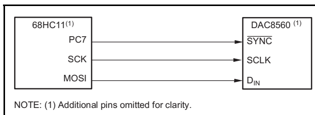
Figure 73. DAC8560 to 68HC11 Interface
