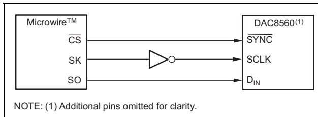
Figure 72. DAC8560 to Microwire Interface
