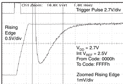
Time (2 \mu S/div)
